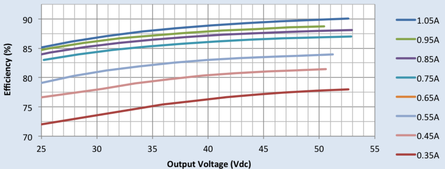
Efficiency vs. Output Voltage at 277Vac @ Tc=70°C
