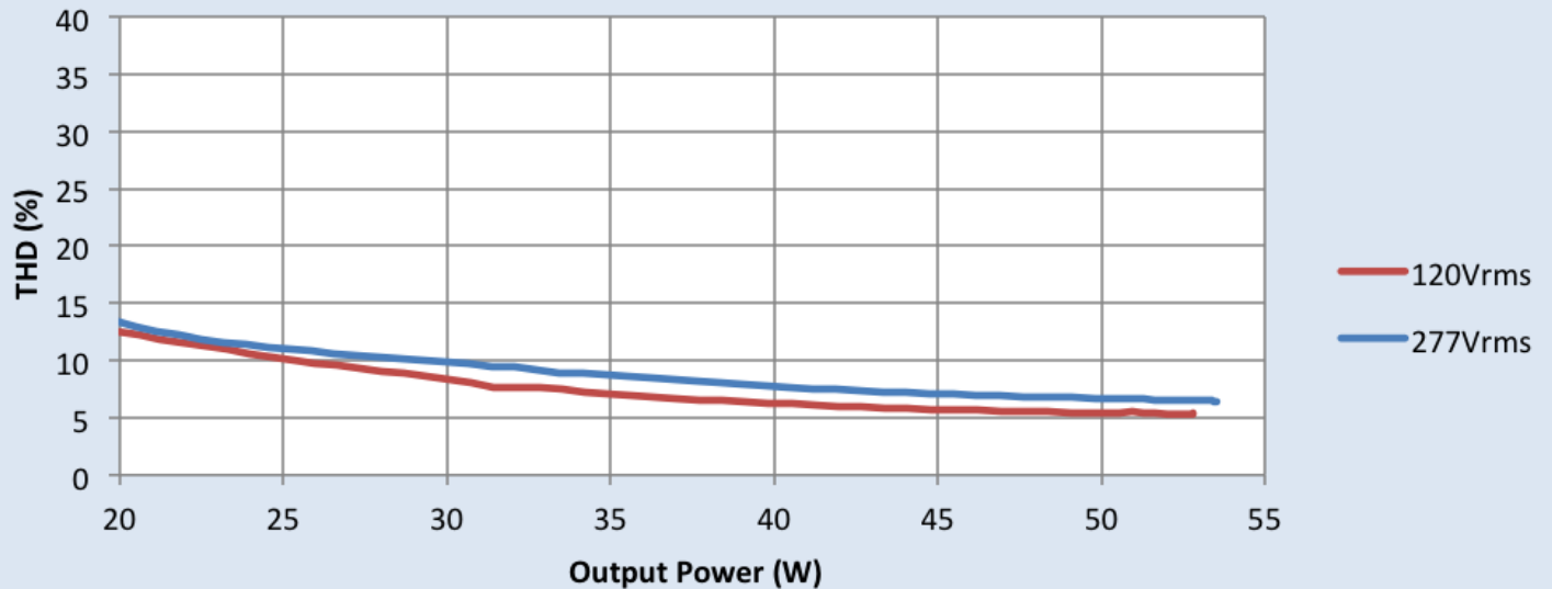
Total Harmonic Distortion vs. Output Power @ Tc=70°C
