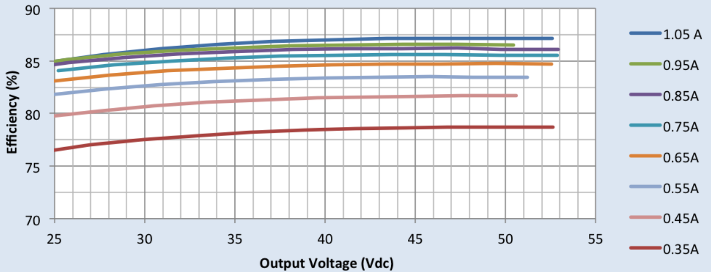
Efficiency vs. Output Voltage at 120Vac @ Tc=70°C
